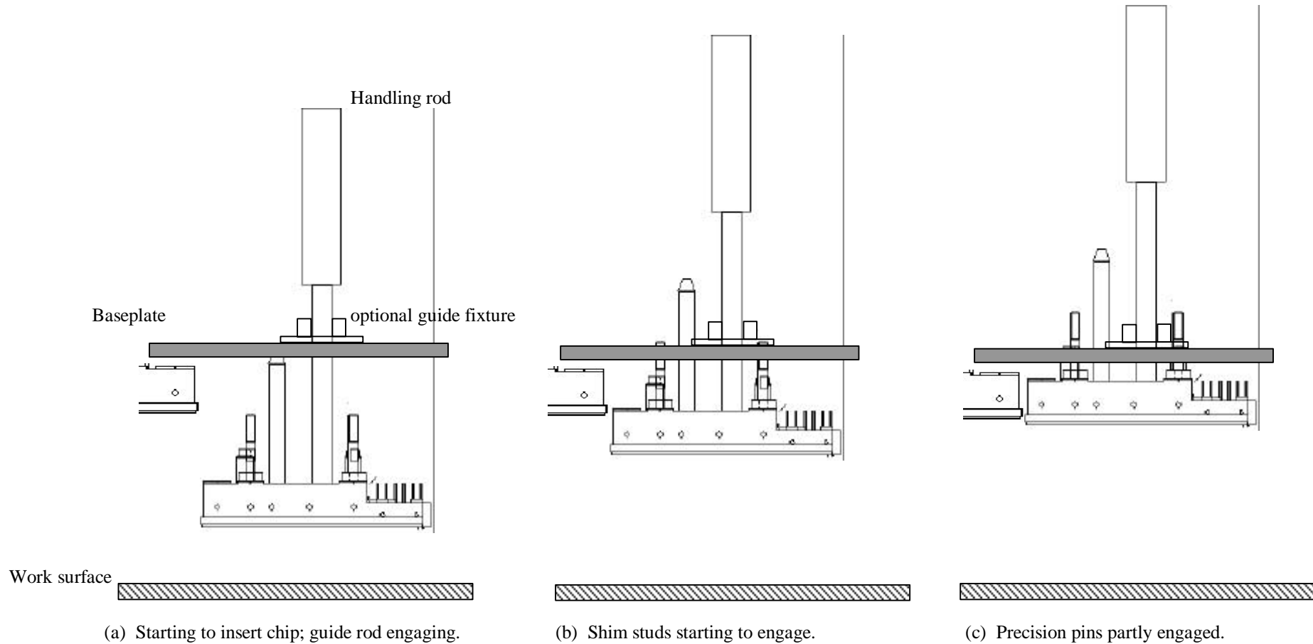
Figure 4. Insertion sequence for CCD into mosaic baseplate.
