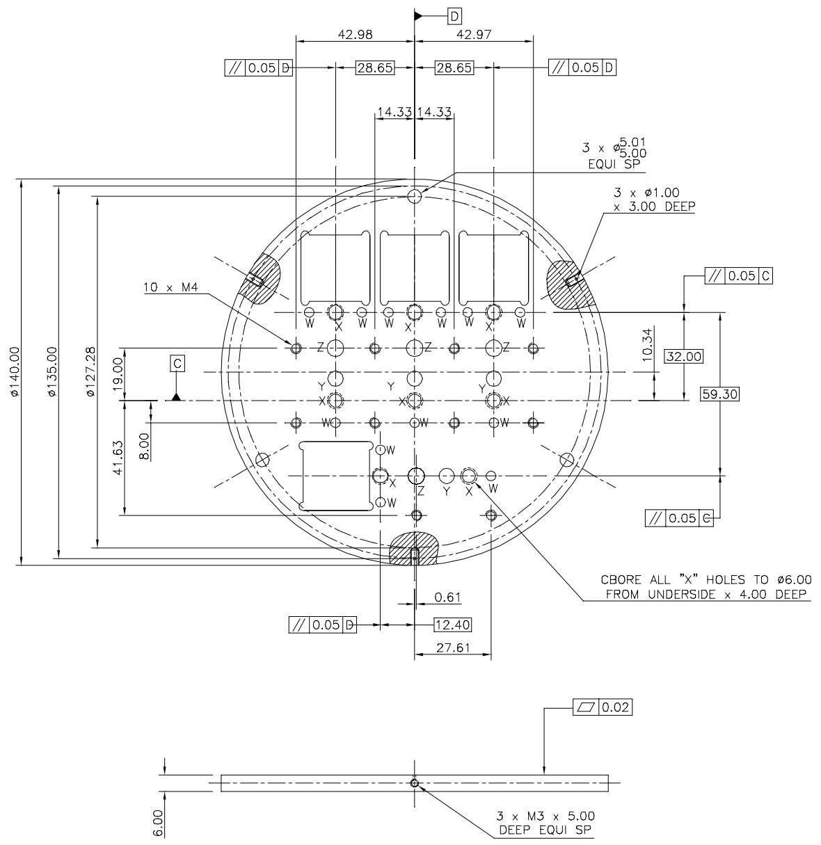
FIGURE 2, AN EXAMPLE OF A CUSTOM INVAR BASEPLATE DESIGNED FOR CRYOGENIC USE OF FOUR CCD42-90'S
